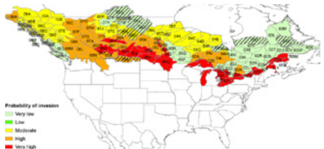
Figure 4. Probability of quagga mussel invasion of Canadian freshwater sub-drainages based on probability of survival and arrival. Hatched watersheds had <5 sampling sites; therefore, a higher level of uncertainty associated with the corresponding invasion probability. (Source: DFO's Risk Assessment for Three Dreissenid Mussels in Canadian Freshwater Ecosystems, 2012 )
